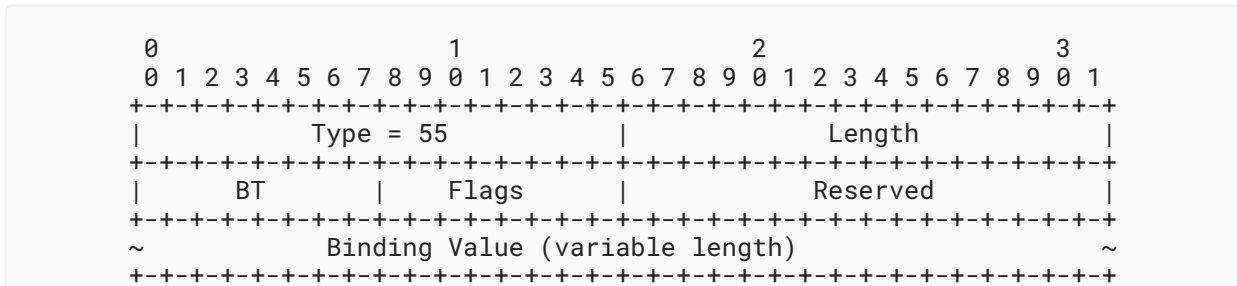
Figure 2: TE-PATH-BINDING TLV
