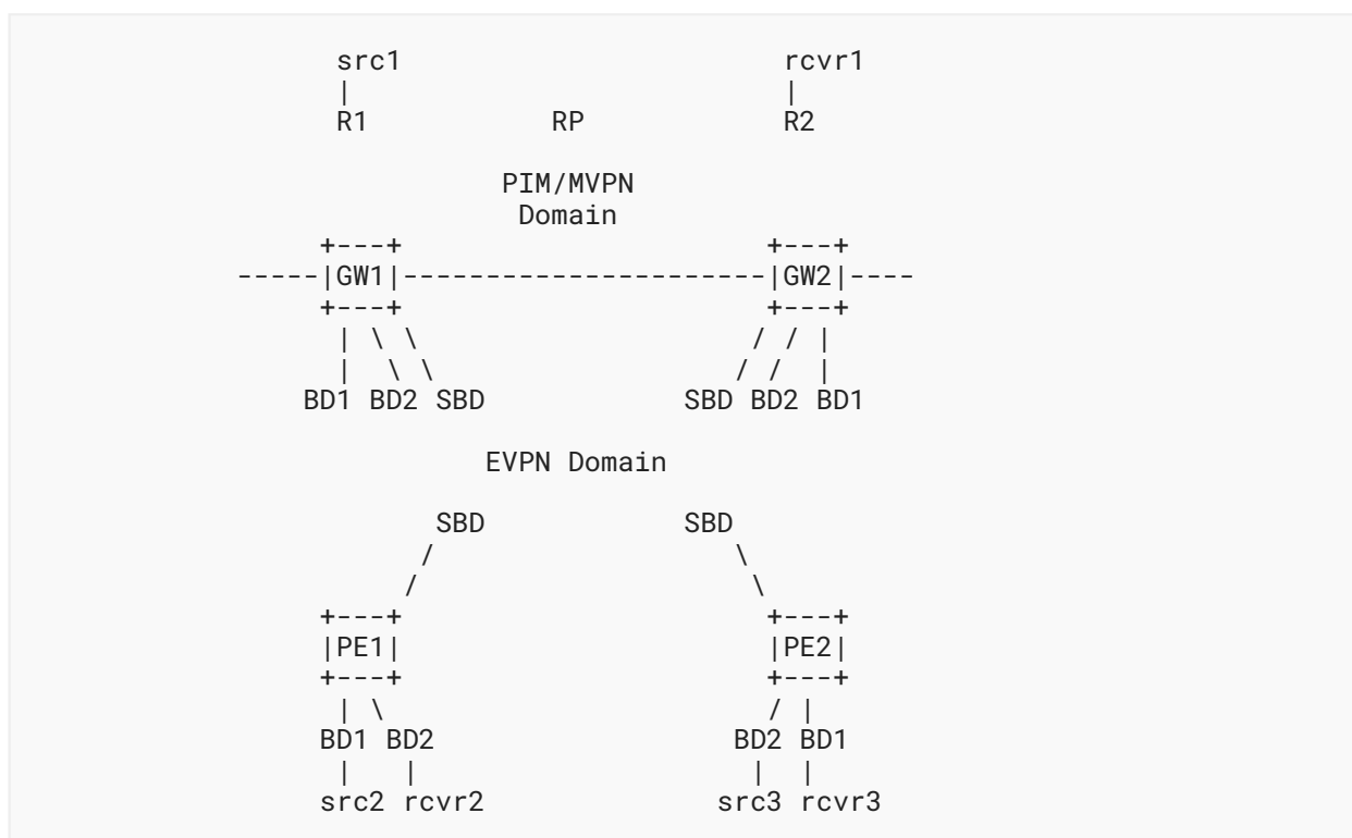
Figure 1: L3 Gateway
