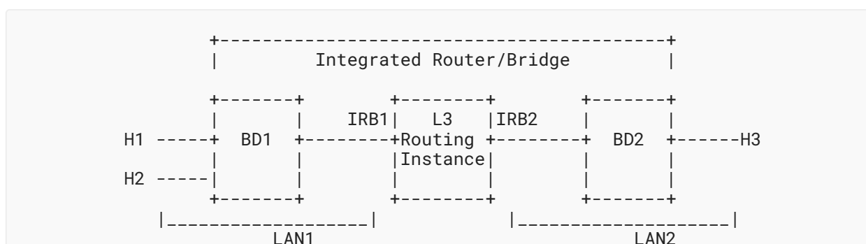
Figure 3: Integrated Router/Bridge
