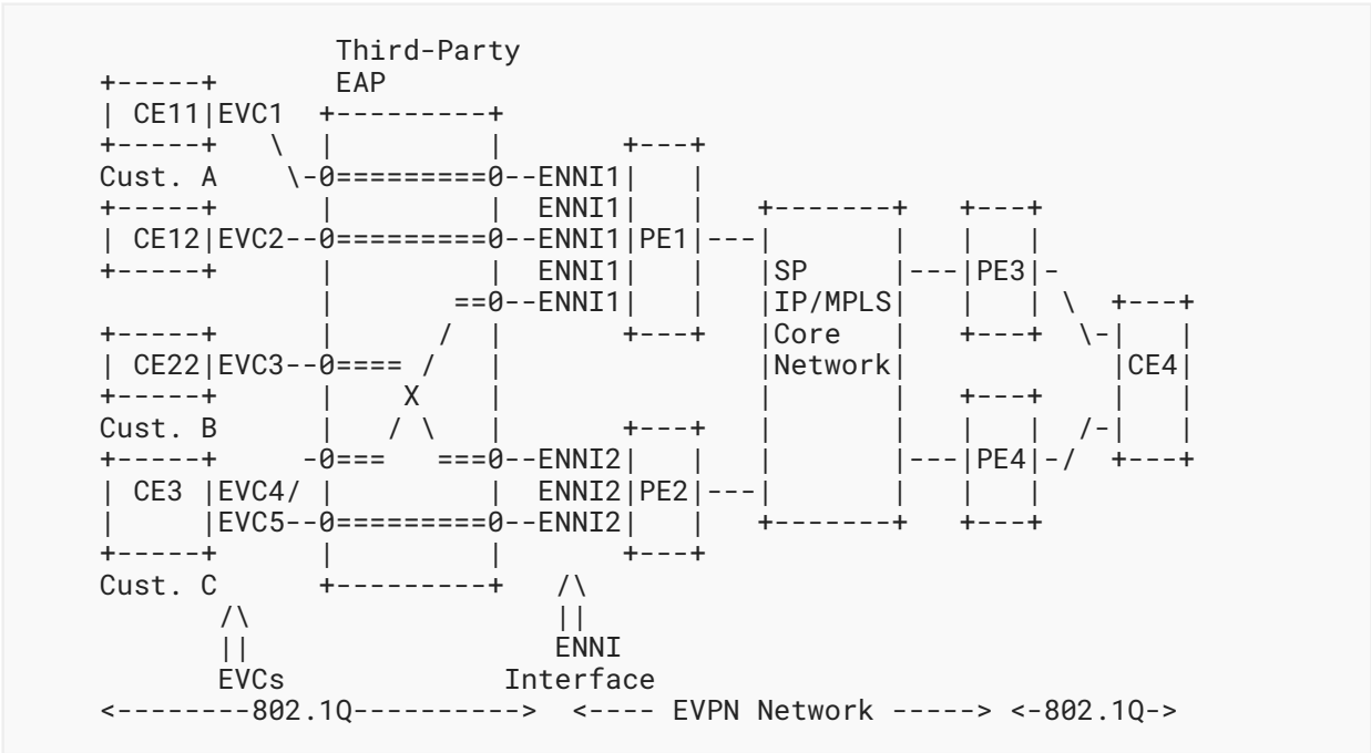
Figure 1: A Dual-Homed Device/Network (Both SA/AA) and SH on the Same ENNI
