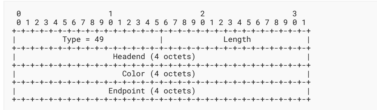
Figure 1: SR Policy Associated PSID - IPv4 Sub-TLV Format
