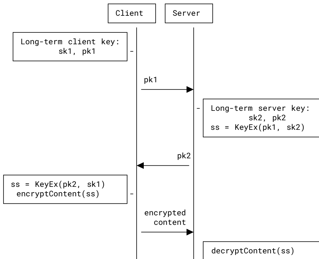
Figure 3: DH-Based AKE
